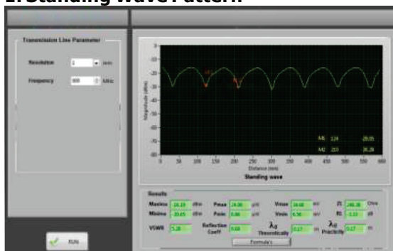
Standing wave @900MHz under OPEN Condition
