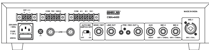
CMA-4400 CENTRAL MIXER AMPLIFIER
