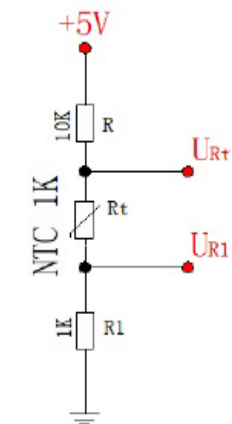
Measurement of thermal resistance
