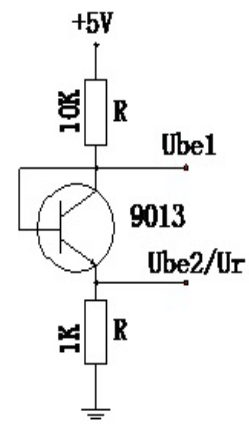
Measurement of PN-junction temperature sensor
