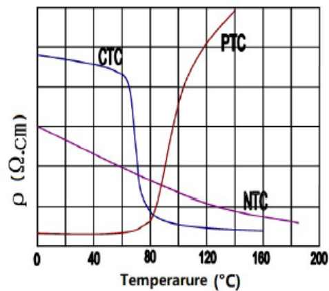
Temperature properties of 3 types of thermal resistances
